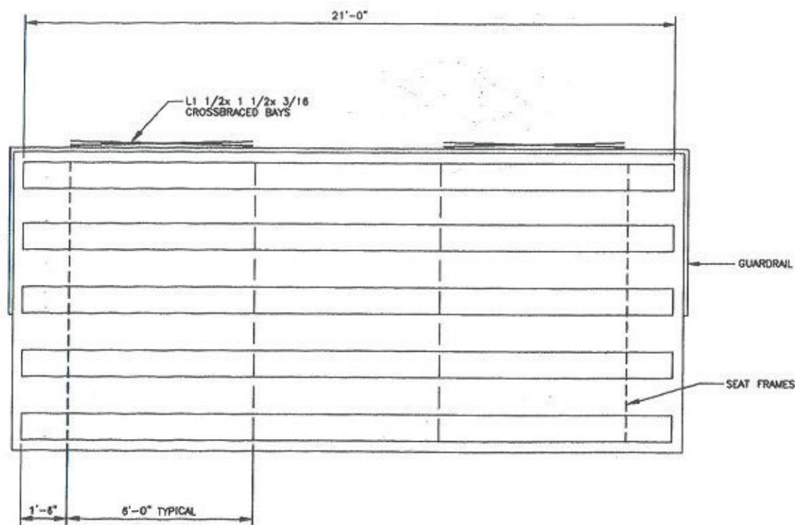
5 ROW SEATING PLAN x 21' & 24'
