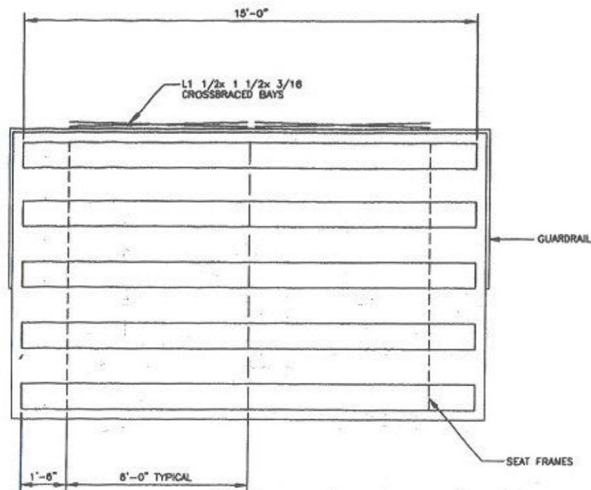
5 ROW SEATING PLAN x 15'
