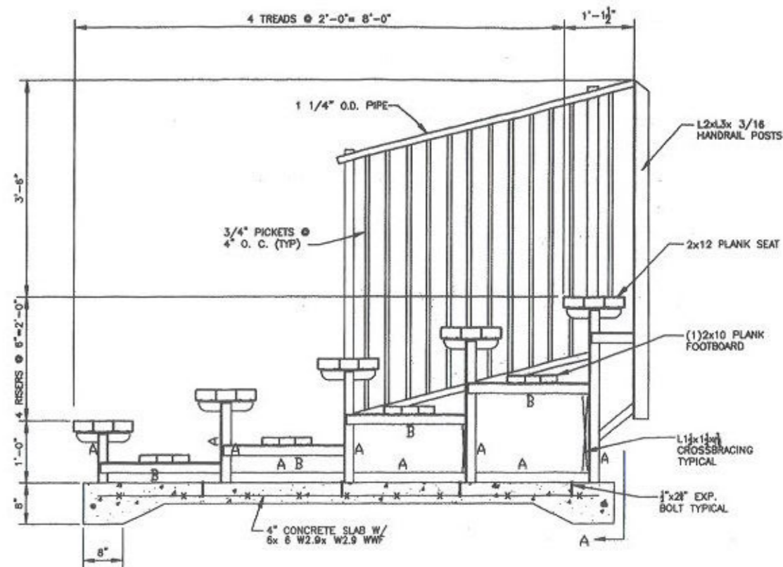
TYPICAL FRAMING ELEVATION
