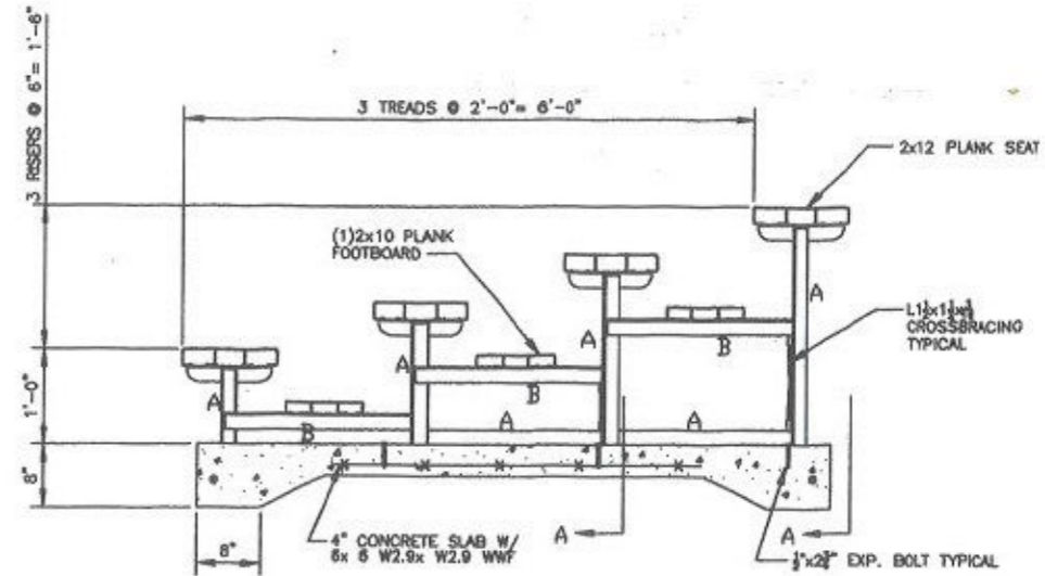
TYPICAL FRAMING ELEVATION SCALE: 1"=1'-0"
