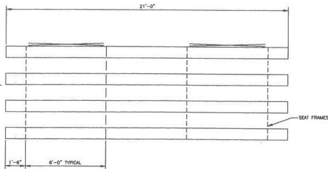
4 ROW SEATING PLAN X 21' SCALE: 1/4"=1'-0"
