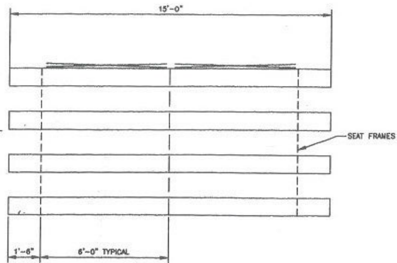
4 ROW SEATING PLAN X 15" SCALE: 1/4"=1'-0"
